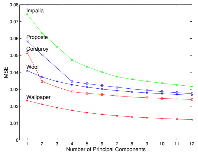
Figure 6: Plot of the reconstruction errors in the Y channel with respect to the number of principal components. This plot indicates that it is sufficient to use eight principal components for most materials we have tested.
