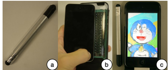
Figure 1: (a) GaussBrush is a magnetic stylus which can be sensed by the (b) thin magnetic sensor grid attached behind a touchscreen device. (c) Sample drawing results by using GaussBrush .
