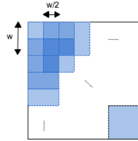
Figure 7: overlapped blocks
