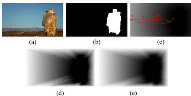
Fig. 7. Generating a saliency distance field. (a) The input image. (b) Saliency region detection [23]. (c) The absolute distance computed from (b) using the Jump Flooding Algorithm. (d) The normalized distance field computed from (c) by replacing d_x with d_x/d_y . (e) Smoothing (d) to eliminate discontinuous artifacts which could be observed around the bottom-right corner.
