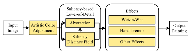
Fig. 2. Pipeline of our image watercolorization.
